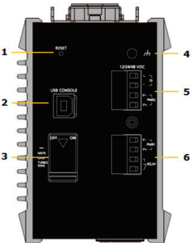
Rear Panel
