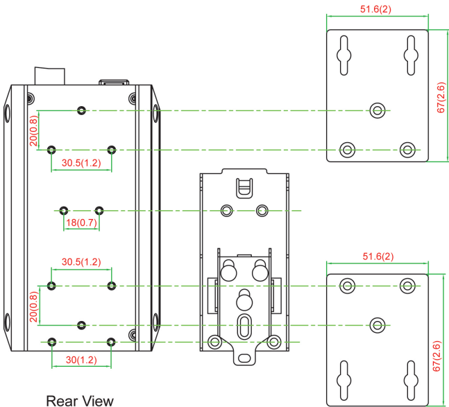
DIN-Rail / Wall Mounting Kit
