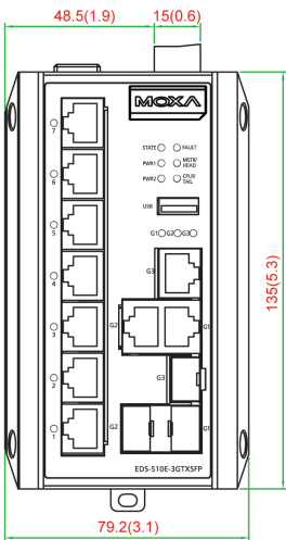
Front View
