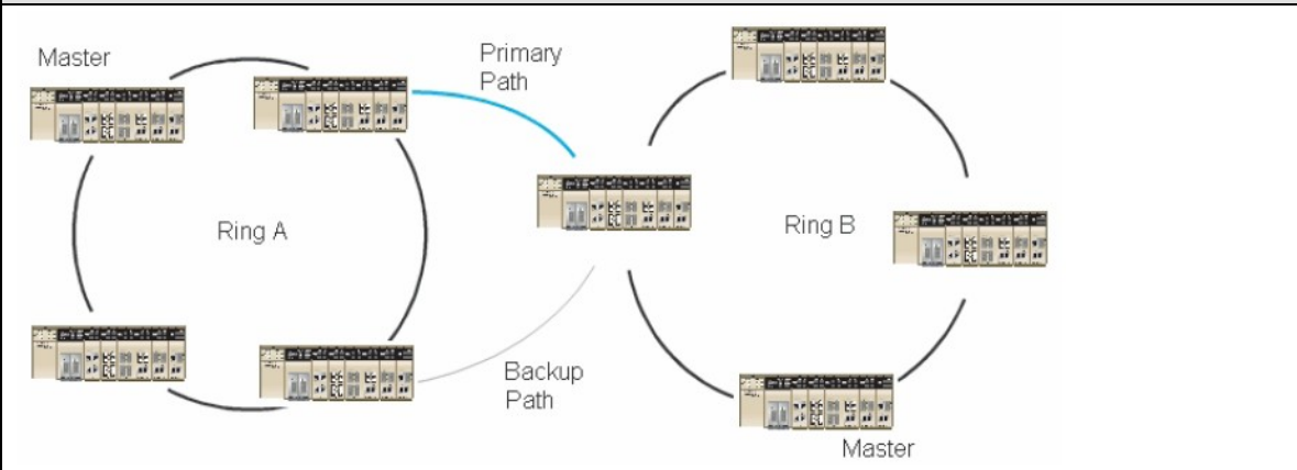
Dual-Homing for a “Turbo Ring V2” Ring.
