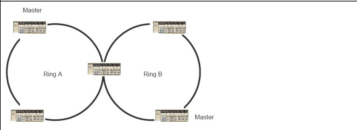
Dual-Ring for a “Turbo Ring V2” Ring.
