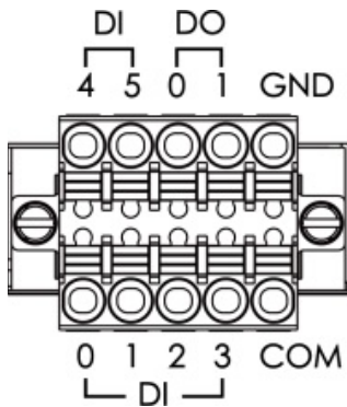
DI's x 6/DO's x 2 (Terminal Block)
